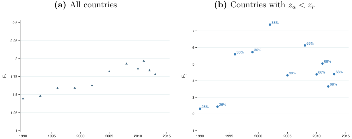
Figure 8: Factor F_0 . 1990-2015.
